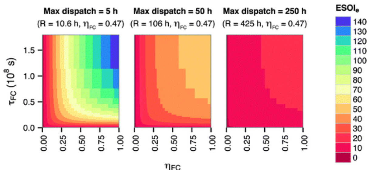
Fig. 4 Dependence of \text{ESOI}_e ratio on \tau_{\text{FC}} , \eta_{\text{FC}} , and R . Calculated from eqn (9) .
