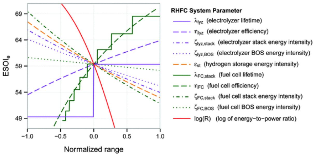
Fig. 3 Dependence of \text{ESOI}_e ratio on individual system parameters. Calculated from eqn (9) . The range of each parameter is specified in Table 3 .
