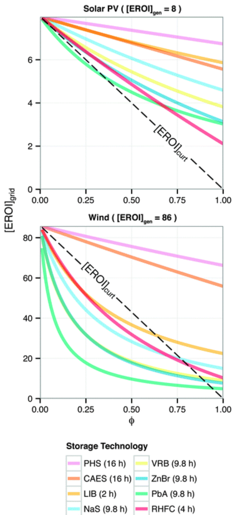
Fig. 7 Energy cost/benefit analysis of storing energy using different storage technologies. Calculated
