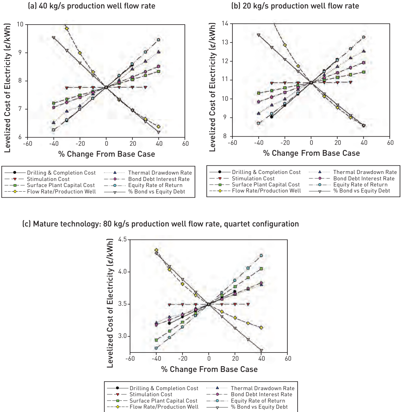
Figure A.9.9 Sensitivity of base case EGS LEC for the Clear Lake (Kelseyville, Calif.) scenario, showing levelized cost of electricity in ¢/kWh for three different production well flow rates.
