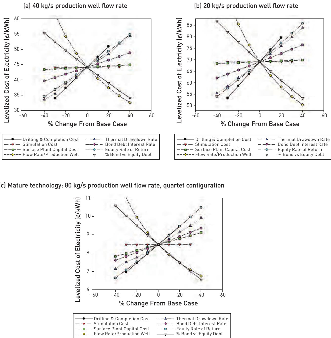
Figure A.9.10 Sensitivity of base case EGS LEC for the Conway, N.H., scenario, showing levelized cost of electricity in ¢/kWh for three different production well flow rates.
