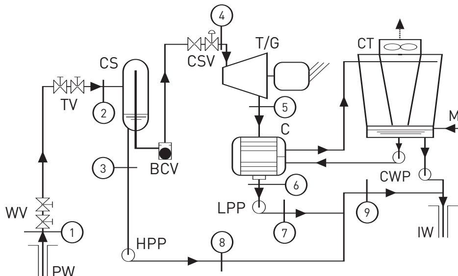
Figure 7.13 Supercritical single-expansion plant with ultra-high inlet pressures.
