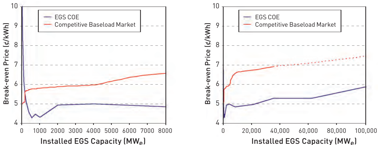
Figure A.9.8 Levelized break-even COE using MIT EGS for the 100,000 MWe - 50 year scenario using a Fixed Charge Rate of 12.8% per the NEMS model. Flow rate per production well (in a triplet configuration – 1 injector, 2 producers) follows the 80 kg/s learning curve. Thermal drawdown is 3%/yr resulting in well-field rework after ~ 6 years. Resulting absorbed technology deployment cost is $262MM U.S. (2004).
