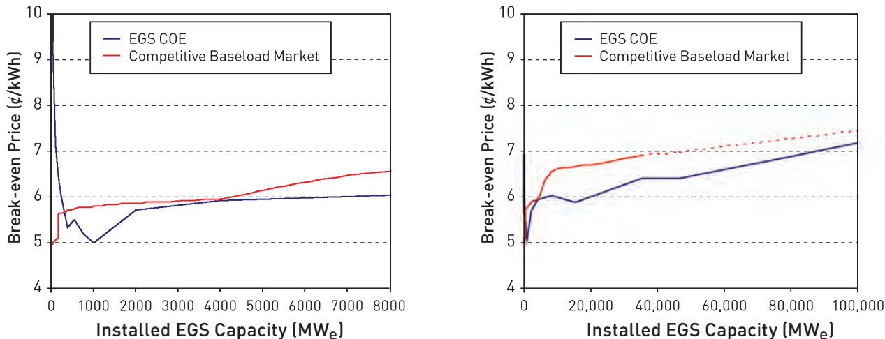
Figure A.9.7 Levelized break-even COE using MIT EGS for the 100,000 MWe - 50 year scenario using a fixed charge rate of 12.8% per the NEMS model. Flow rate per production well (in a triplet configuration – 1 injector, 2 producers) follows the 60 kg/s learning curve. Thermal drawdown is 3%/yr resulting in well-field rework after ~ 6 years. Resulting absorbed technology deployment cost is $368MM U.S. (2004).
