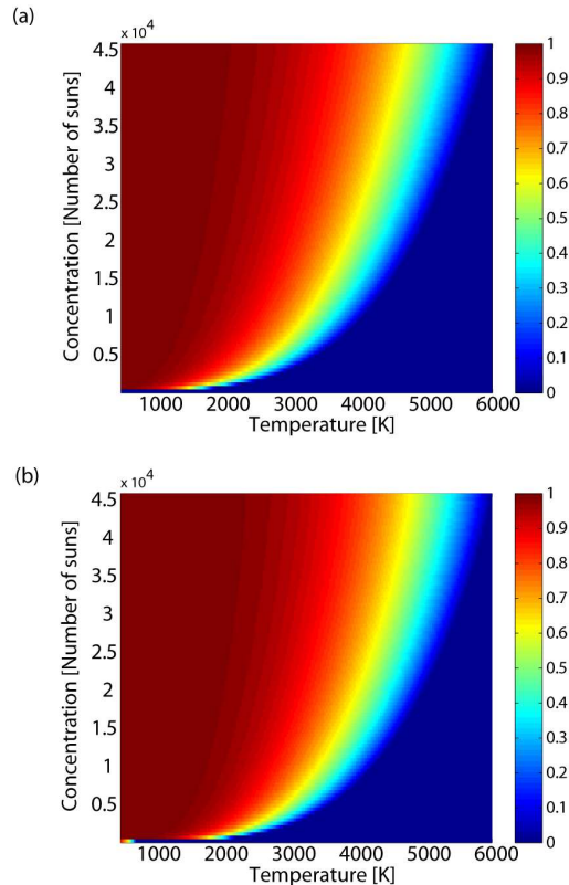
Fig. 2. Intermediate efficiency ( \eta_i ) vs. solar concentration (Ns) and equilibrium temperature (T) for: (a) Blackbody absorber. (b) Pyramid array absorber in Fig. 1(b), assuming an ideal solar spectrum with the solar temperature set at 6000K.
