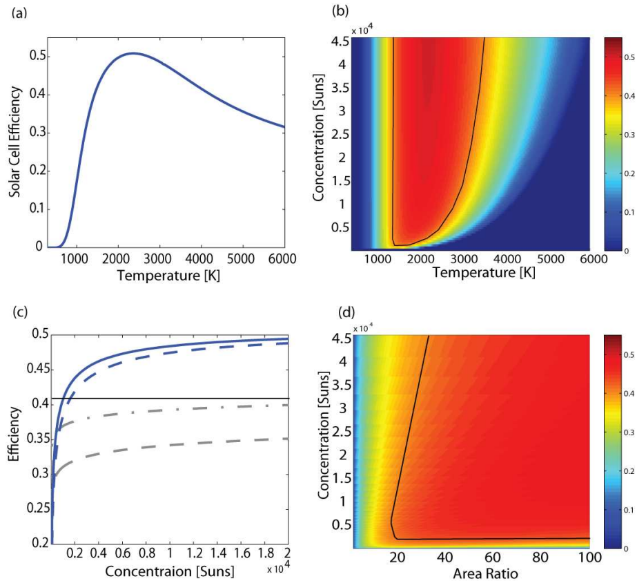
Fig. 6. (a) Efficiency \eta_{SC} of a 0.7[eV] solar cell exposed to radiation from our emitter shown in Fig. 1(c). (b) STPV system efficiency vs. temperature and concentration (black contour indicates the SQ limit at 41%.) (c) System efficiency vs. concentration, blue curve: maximum STPV system efficiency using our absorber and emitter pair and a 0.7[eV] solar cell (Ideal 6000K blackbody—solid line; AM 1.5 spectrum—dashed line); Grey curves: Dashed—efficiency of a 0.7[eV] cell; Dashed-dotted—efficiency of a 1.1[eV] cell, both when directly exposed to sunlight; Black line: theoretical limit of 41% in SQ analysis. (d) STPV system efficiency vs. area ratio and concentration (black contour indicates the SQ limit.)
