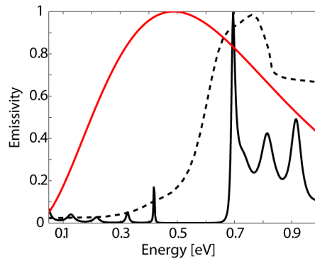
Fig. 5. Properties of the emitter, shown in Fig. 1(c), that consists of a Tungsten slab and a multilayer dielectric stack. (a) Emissivity (averaged over both polarizations) vs. polar angle and energy. (b) The black curve is the emissivity of our emitter structure at normal incidence ( \theta = 0 ). The dashed black curve is the emissivity at normal incidence of a tungsten crossed grating structure ( 1.5\mu\text{m} period; 1\mu\text{m} hole width; 400\text{nm} hole depth). The red curve is the scaled spectral radiance of a 2000K blackbody.
