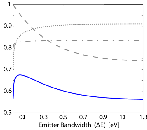
Fig. 4. Solar cell \eta_{sc} (blue curve) and its three components: U(T, E_g) (dashed curve), v(T, E_g) (dotted curve), and m(V_{op}) (dashed-dotted curve), for the case of an idealized emitter at T = 2000\text{K} with emissivity: \varepsilon_{ideal}(\Delta E) = \Theta(E - E_g) - \Theta(E - E_g - \Delta E) with E_g = 0.7[\text{eV}]
